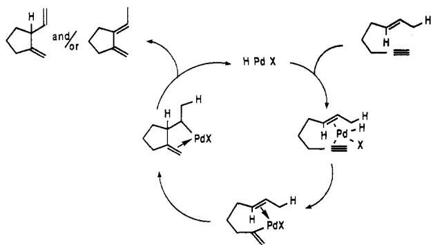
Scheme II Hydropalladation Reaction Pathway
